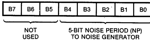
Fig. 7-5. Noise Period Register. (Courtesy General Instrument Corp.)
